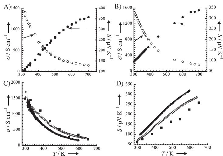
Figure 1. Temperature dependence of the electrical conductivity \sigma ( \circ ) and the Seebeck coefficient S ( \bullet ) for A) \text{Na}_{0.95}\text{Pb}_{19}\text{SbTe}_{21} and B) \text{Na}_{0.95}\text{Pb}_{20}\text{SbTe}_{22} . Temperature dependence of C) the electrical conductivity \sigma and D) the Seebeck coefficient S for \text{Na}_{0.8}\text{Pb}_{20}\text{Sb}_y\text{Te}_{22} with y = 0.4 ( \blacksquare ), 0.6 ( \circ ), and 0.8 ( \blacktriangle ). The conductivity and thermopower measurements were performed simultaneously on samples of typical size 7 \times 5 \times 4 \text{ mm}^3 . See Supporting Information for measurement details. [28]
