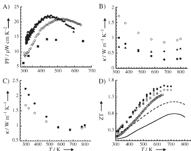
Figure 2. A) Temperature dependence of the power factor \text{PF} = \sigma S^2 for \text{Na}_{0.8}\text{Pb}_{20}\text{Sb}_y\text{Te}_{22} with y = 0.4 ( \blacksquare ), 0.6 ( \circ ), and 0.8 ( \blacktriangle ). B) Temperature dependence of the thermal conductivity \kappa of \text{Na}_{0.95}\text{Pb}_{20}\text{SbTe}_{22} ( \circ ), showing the lattice \kappa_{\text{latt}} ( \blacktriangle ) and carrier \kappa_{\text{el}} ( \bullet ) contributions. See text for details. C) Temperature dependence of the thermal conductivity \kappa of \text{Na}_{0.95}\text{Pb}_{19}\text{SbTe}_{21} ( \circ ) and \text{Na}_{0.8}\text{Pb}_{20}\text{Sb}_{0.6}\text{Te}_{22} ( \bullet ). D) Temperature dependence of the thermoelectric figure of merit \text{ZT} for \text{Na}_{0.95}\text{Pb}_{20}\text{SbTe}_{22} ( \bullet ), \text{Na}_{0.95}\text{Pb}_{19}\text{SbTe}_{21} ( \circ ), and \text{Na}_{0.8}\text{Pb}_{20}\text{Sb}_{0.6}\text{Te}_{22} ( \square ), compared to those of the state-of-the-art p-type materials \text{PbTe} (solid line) and TAGS (dashed line). See Supporting Information for measurement details. [28]
