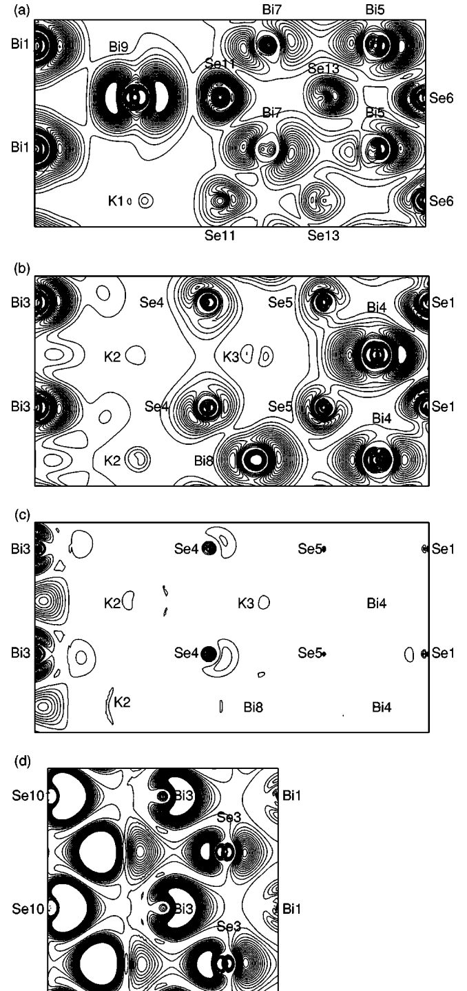
FIG. 9. Charge density of \beta\text{-K}_2\text{Bi}_8\text{Se}_{13} supercell in planes parallel to the c axis corresponding to (a),(b) CBM states and (c),(d) VBM states. The charge density is represented by closed lines from low charge density regions to high charge density regions in steps of 5 \times 10^{-4} electrons/ \text{\AA}^3 .
