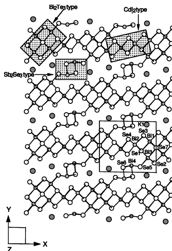
FIG. 1. Projection of the crystal structure of \alpha - \text{K}_2\text{Bi}_8\text{Se}_{13} viewed down the c axis ( z axis). \text{Bi}_2\text{Te}_3 , \text{CdI}_2 and \text{Sb}_2\text{Se}_3 building blocks in the structure are highlighted by the shaded areas.
