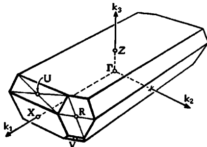
FIG. 3. Brillouin zone of \alpha - K_2Bi_8Se_{13} .
