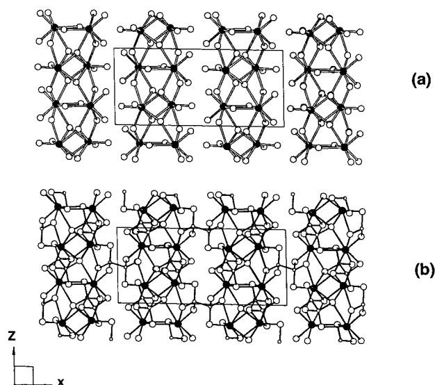
Figure 5. Structure of \alpha\text{-Bi}_4(\text{P}_2\text{Se}_6)_3 (adapted from ref 9): (a) infinite [\text{Bi}_4\text{Se}_{18}] layers running along the bc plane; (b) view along the b axis of the \alpha\text{-Bi}_4(\text{P}_2\text{Se}_6)_3 structure showing the interlayer bonding through the phosphorus pairs. Atom identifications are the same as those of Figure 4.
