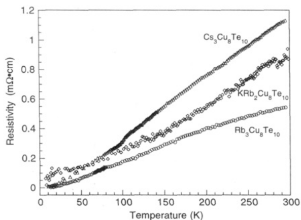
Figure 8. Variable-temperature four-probe resistivity data measured on single crystals of (A) Rb_3Cu_8Te_{10} , (B) Cs_3Cu_8Te_{10} , and (C) KRb_2Cu_8Te_{10} .
