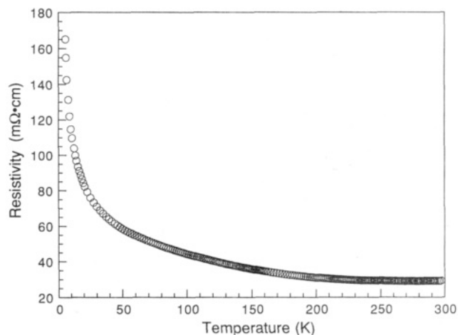
Figure 10. Variable-temperature four-probe resistivity data measured on a single crystals of Rb_2BaCu_8Te_{10} .
