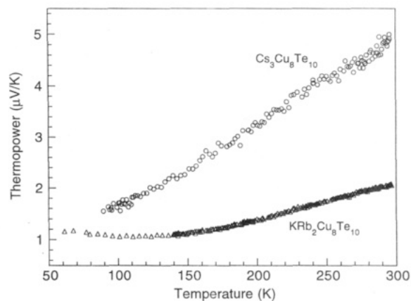
Figure 9. Variable-temperature thermoelectric power data measured on single crystals of (A) Rb_3Cu_8Te_{10} , (B) Cs_3Cu_8Te_{10} , and (C) KRb_2Cu_8Te_{10} .
