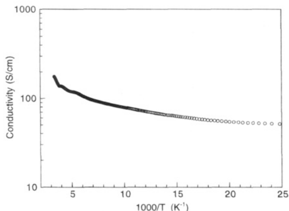
Figure 7. Single crystal variable-temperature four-probe resistivity data for K_4Cu_8Te_{11} .
