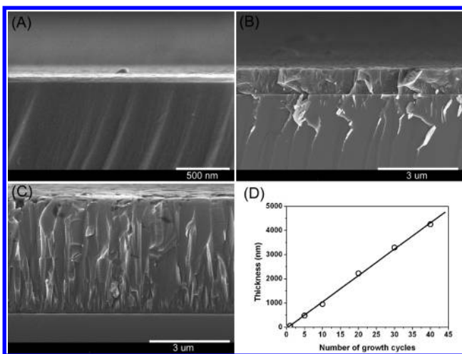
Figure 1. Cross-sectional SEM images of ZIF-8 films grown on silicon substrates with cycles of (A) 1, (B) 10, and (C) 40; (D) thickness of ZIF-8 film versus numbers of growth cycles.
