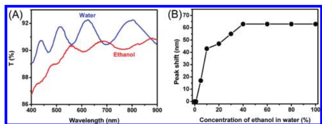
Figure 4. (A) UV-vis transmission spectra of 10-cycle ZIF-8 film grown on glass substrate on exposure to vapors of ethanol and water. (B) Interference peak (originally at 612 nm) shift versus ethanol concentration in ethanol/water solutions. The concentration is expressed as a volume percentage.
