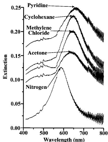
Figure 14. Extinction spectra of aspect ratio 2.17 Ag SL PPA measured in various solvents. Spectra have been arbitrarily spaced along the extinction axis for clarity.
