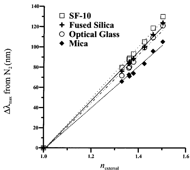
Figure 18. LSPR peak shift from dry \text{N}_2 versus the refractive index of the solvent, n_{\text{external}} , for each of the four substrates. The plotted points represent the average shift recorded for several samples of each substrate. Each data set was fit to a line with the following equations: fused silica, y = 238x - 241 ; borosilicate glass, y = 229x - 230 ; mica, y = 206x - 208 ; SF-10, y = 258x - 259 .
