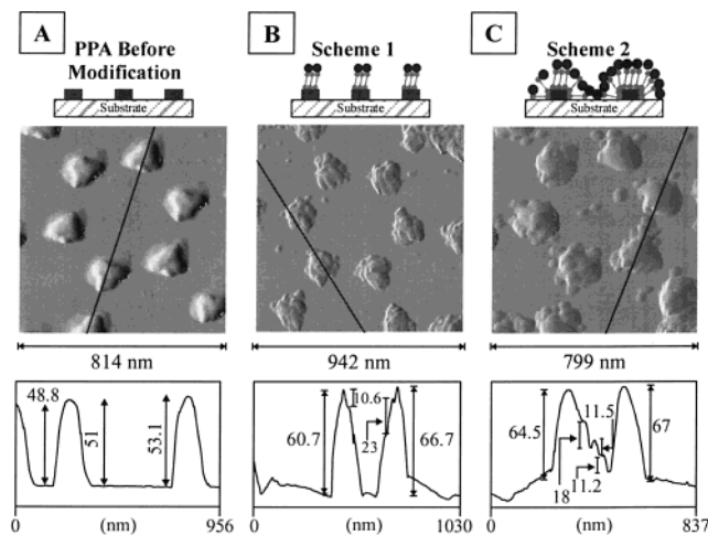
Figure 4. Schematic illustrations and tapping mode AFM images of colloid-modified SL PPA samples ( D = 400 nm and d_m = 50 nm). (A) Unmodified Ag SL PPA, (B) top face only modification of Ag SL PPA with 13 nm diameter Au colloids, and (C) four face modification of Ag SL PPA with 13 nm diameter Au colloids.
