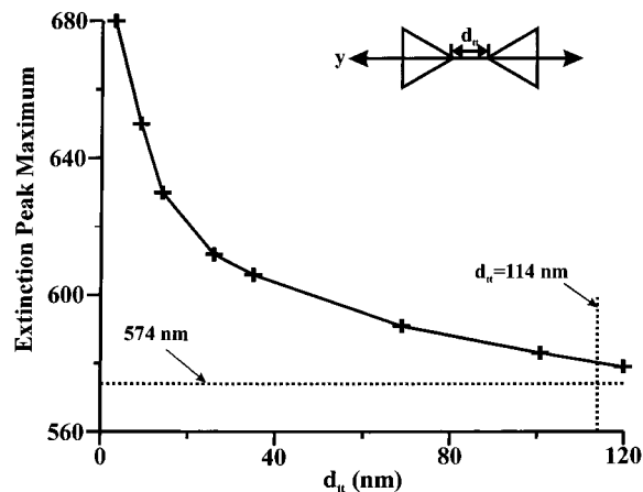
Figure 13. Effect of nanoparticle–nanoparticle interaction on the extinction spectrum of two truncated tetrahedra. The extinction peak maximum is plotted as a function of d_{tt} . Results are calculated using the discrete dipole approximation with 10 234 dipoles in each nanoparticle, dielectric constants from Palik, and polarization along the y axis. The solid lines are a guide for the eye.
