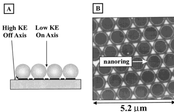
Figure 3. Schematic illustration (A) and representative AFM image (B) of nanoring and SL PPA fabrication. The ambient contact mode AFM image was captured from a sample fabricated with D = 979 nm nanospheres and d_m = 50 nm e-beam deposited Ni metal after three minutes sonication in methylene chloride.
