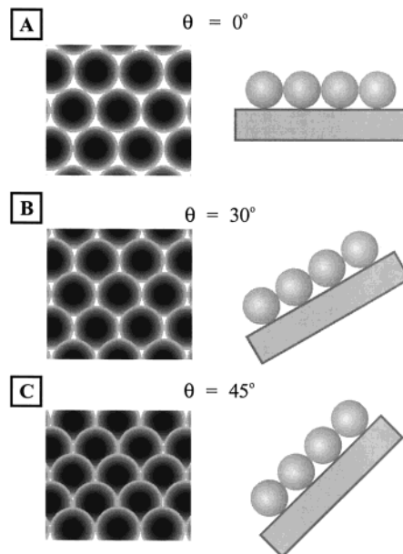
Figure 5. Schematic of the angle resolved deposition process. (A) Samples viewed at 0^\circ . The interstices in the nanosphere mask are equally spaced and of equal size. (B) Sample viewed at 30^\circ . The interstices in the nanosphere mask follow a pattern including two different interparticle spacing values, and the interstitial area is smaller. (C) Sample viewed at 45^\circ . The interstices are now closed to line of sight deposition.
