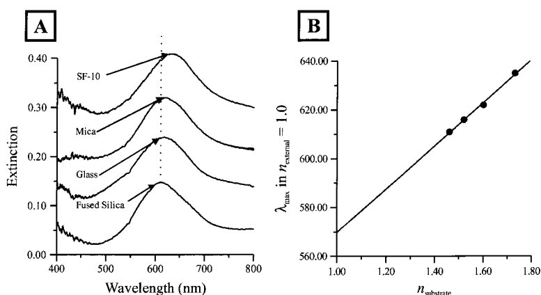
Figure 17. Effect of substrate refractive index on LSPR \lambda_{\text{max}} . (A) UV-visible extinction spectra for a Ag SL PPA ( D = 400 nm and d_m = 25 nm) on various substrates. (B) LSPR \lambda_{\text{max}} of Ag SL PPA in a \text{N}_2 environment versus the refractive index of the substrate, n_{\text{substrate}} . Linear regression was used to fit the data to a line described by the following equation: y = 87x + 483.5 .
