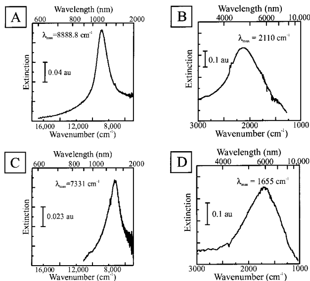
Figure 12. Near/mid infrared extinction spectra of Ag SL PPA on varied substrates. Reported spectra are raw, unfiltered data. (A) D = 820 \pm 15 nm, d_m = 20 nm, glass substrate; (B) D = 2700 \pm 70 nm, d_m = 65 nm, silicon substrate; (C) D = 1100 \pm 15 nm, d_m = 25 nm, glass substrate; (D) D = 2542 \pm 80 nm, d_m = 50 nm, germanium substrate.
