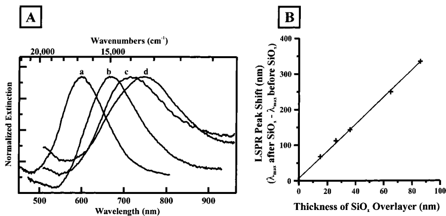
Figure 16. Effect of \text{SiO}_x overlayer thickness on LSPR \lambda_{\text{max}} . (A) UV-visible extinction spectra for a Ag SL PPA sample ( D = 400 nm and d_m = 25 nm) on glass with various \text{SiO}_x overlayer thickness: (a) No \text{SiO}_x overlayer; \lambda_{\text{max}} = 597 nm, (b) \text{SiO}_x overlayer thickness = 15 nm; \lambda_{\text{max}} = 669 nm, (c) \text{SiO}_x overlayer thickness = 26 nm; \lambda_{\text{max}} = 714 nm; (d) \text{SiO}_x overlayer thickness = 36 nm; \lambda_{\text{max}} = 745 nm. (B) Plot of LSPR peak shift, \Delta\lambda_{\text{max}} , versus \text{SiO}_x overlayer thickness. The slope of the linear fit of the data indicates that \lambda_{\text{max}} shifts to the red 4 nm for every 1 nm of deposited \text{SiO}_x .
