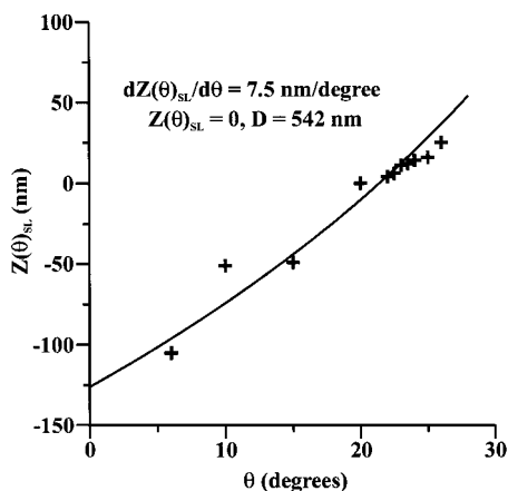
Figure 8. Plot of the predicted nanooverlap/nanogap, Z(\theta)_{SL} , as a function of angle assuming a nanosphere size D equal to 542 nm. At the point where Z(\theta)_{SL} is equal to 0 nm ( \theta = 21.42^\circ ), the derivative of the curve is equal to 7.5 nm/degree.
