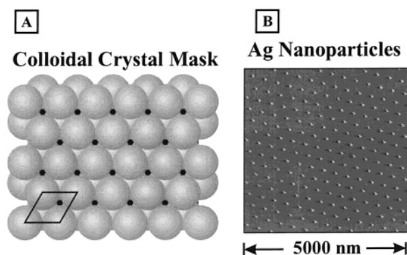
Figure 2. Schematic illustration (A) and representative AFM image (B) of DL PPA. The ambient contact mode AFM image was captured from a SL PPA fabricated with D = 400 nm nanospheres and d_m = 30 nm thermally evaporated Ag metal after three minutes sonication in methylene chloride.
