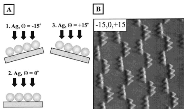
Figure 9. Schematic illustration (A) and contact mode AFM image (B) of three deposition nanochain structure on mica. 1.6 \mu\text{m} \times 1.6 \mu\text{m} area, D = 542 \text{ nm} , d_m = 10 \text{ nm} , \theta_{\text{dep}} = +15^\circ, 0^\circ , and -15^\circ .
