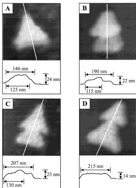
Figure 6. Contact mode AFM images of Ag SL PPA nanooverlap structures fabricated on mica substrates. All reported line scan values have not been deconvoluted for tip broadening effects. (A) 300 nm \times 300 nm image, D = 542 nm, d_m = 20 nm, \theta_{\text{dep}} = 0^\circ and 6^\circ . (B) 250 nm \times 250 nm image, D = 542 nm, d_m = 20 nm, \theta_{\text{dep}} = 0^\circ and 10^\circ . (C) 300 nm \times 300 nm image, D = 542 nm, d_m = 20 nm, \theta_{\text{dep}} = 0^\circ and 15^\circ . (D) 250 nm \times 250 nm image, D = 542 nm, d_m = 20 nm, \theta_{\text{dep}} = 0^\circ and 20^\circ .
