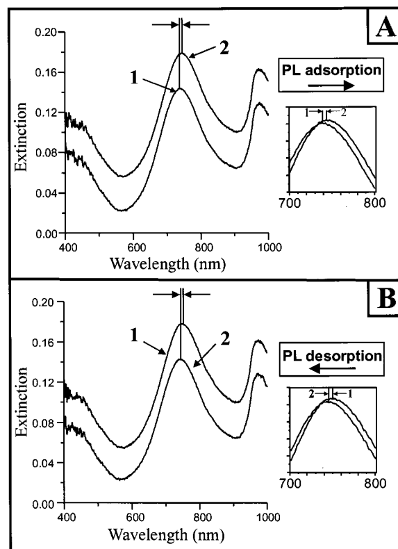
Figure 21. LSPR detected absorption/desorption of PL to 11-MUA/1-OT mixed SAM. (A) PL adsorption. 1. Extinction spectrum of 11-MUA/1-OT modified Ag nanoparticles ( D = 400 nm and d_m = 50 nm) in 5 mM phosphate buffer, pH = 8.5; \lambda_{\max} = 744.6 nm. 2. Extinction spectrum after incubation with PL (1 mM in lysine); \lambda_{\max} = 749.8 nm. (B) PL desorption. 1. Extinction spectrum of 11-MUA/1-OT modified Ag nanoparticles with adsorbed PL in 5 mM phosphate buffer, pH = 8.5; \lambda_{\max} = 749.8 nm. 2. Extinction spectrum after introducing high ionic strength buffer (20 mM phosphate buffered saline; 278 mM NaCl; 5.7 mM KCl); \lambda_{\max} = 744.9 nm.
