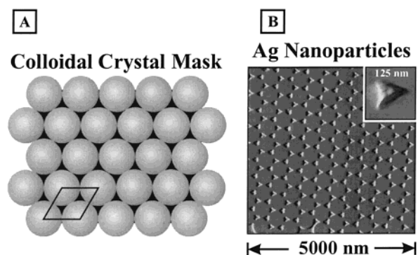
Figure 1. Schematic illustration (A) and representative AFM image (B) of SL PPA. The ambient contact mode AFM image was captured from a SL PPA fabricated with D = 542 nm nanospheres and d_m = 48 nm thermally evaporated Ag metal after 3 min sonication in methylene chloride.
