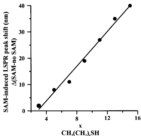
Figure 19. Alkanethiol chain length dependence on LSPR spectral peak shift. All extinction measurements were collected in a N_2 environment. Linear regression was used to fit the data to a line described by the following equation: y = 3.3x - 9.3 .
