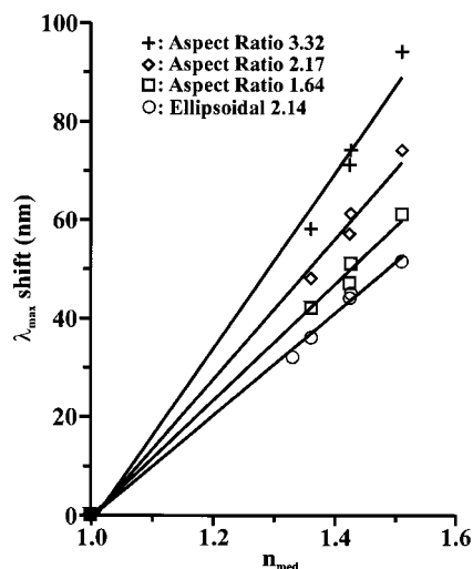
Figure 15. LSPR \lambda_{\max}(\text{solvent}) - \lambda_{\max}(\text{dry N}_2) versus the refractive index of the solvent for unannealed aspect ratios 3.32, 2.17, and 1.64 and annealed aspect ratio 2.14 Ag SL PPA samples.
