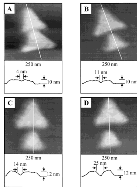
Figure 7. Contact mode AFM images of Ag SL PPA nanogap structures fabricated on mica substrates. All reported line scan values have not been deconvoluted for tip broadening effects. (A) 250 nm \times 250 nm image, D = 542 nm, d_m = 20 nm, \theta_{\text{dep}} = 0^\circ and 22^\circ . (B) 250 nm \times 250 nm image, D = 542 nm, d_m = 20 nm, \theta_{\text{dep}} = 0^\circ and 23^\circ . (C) 250 nm \times 250 nm image, D = 542 nm, d_m = 20 nm, \theta_{\text{dep}} = 0^\circ and 24^\circ . (D) 250 nm \times 250 nm image, D = 542 nm, d_m = 20 nm, \theta_{\text{dep}} = 0^\circ and 26^\circ .
