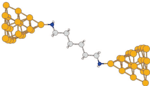
Figure 1. Representative tunnel junction model: depicted is the \text{Au}_{20}\text{-NH}_2\text{-(SiH}_2)_6\text{-NH}_2\text{-Au}_{20} junction. An additional 5 \times 5 layer of gold atoms (not shown) is placed on either side of the above junction for the NEGF/DFT calculations to allow for periodic DFT calculations.
