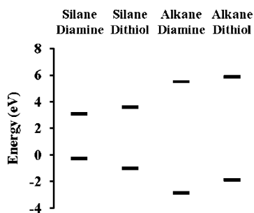
Figure 6. Molecular frontier energy levels for the hexane and hexasilane bonded to gold clusters via amine and thiol end groups. Energies levels are approximated by the Kohn–Sham eigenvalues from the DFT/B3LYP calculations described in the text. The zero of energy is taken to be the Fermi level approximated as the work function of gold ( -5.1 eV). 52 The band gaps of the silane chains are much smaller than the band gaps of the alkane chains, leading to lower \beta decay values for the silanes.
