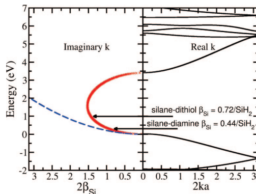
Figure 8. Similar to Figure 7, but for silicon hydride chains and silane-based tunnel junctions with amine or thiol linkers. The substantially decreased HOMO–LUMO gap size in the silanes, compared to the alkanes (Figure 7), makes the values of \beta_{\text{Si}} more sensitive to small differences in the Fermi-level alignment.
