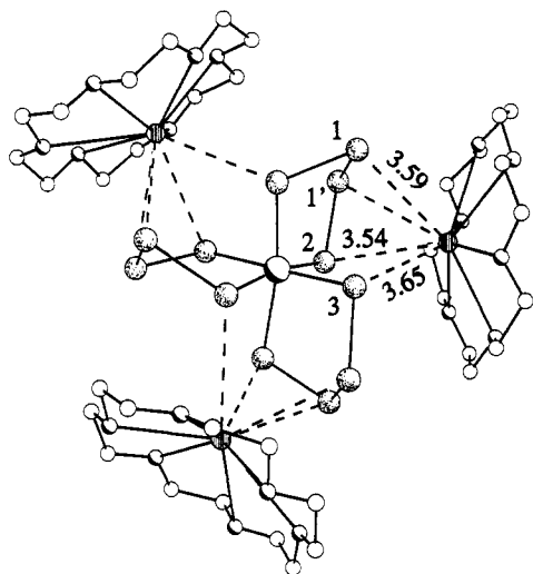
Figure 2. Part of the crystal structure of [\text{K}(\text{18-crown-6})]_3[\text{Ir}(\text{Se}_4)_3] . The orientation of the cations, the interactions of \text{K}^+ ions with the Se atoms, and relevant distances are shown. Hydrogen atoms have been omitted for the sake of clarity.
