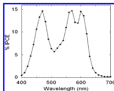
Figure 2. IPCE measured over 10 nm intervals for 2a on 60- \mu\text{m} -thick ZnO nanotube photoanodes. The dye deposition time is 20 min.
