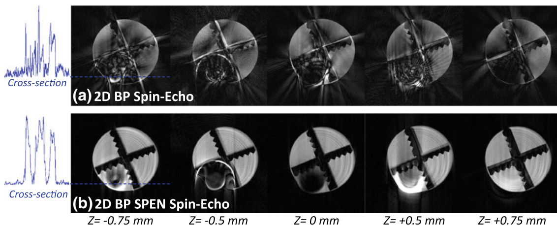
Fig. 3 Idem as in Fig. 2, but upon utilizing the back-projected sequence variants introduced in Fig. 1c, d. Projections were performed by varying the x - and y -gradient strengths so as to provide
