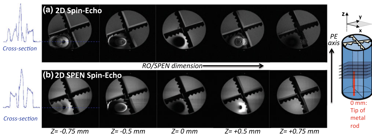
Fig. 2 Comparison of multi-shot MR images of a metal-implanted cross-shaped phantom shown at the right side of the figure and using a Cartesian sampling scheme. a Results obtained from the k -space encoded spin echo sequence illustrated in Fig. 1a; b Idem for the SPEN-based sequence illustrated in Fig. 1b. Slices along the vertical z direction were selected at the indicated positions by changing the offset of the slice-selective RF pulses in the sequences. In both data
