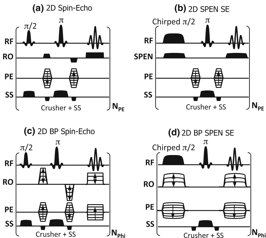
Fig. 1 Multi-shot 2D MRI pulse sequences compared in the present study. a, b Conventional k -encoded spin echo and new SPEN-based spin echo sequence proposed in this study. In the experiments described below, both sequences were implemented with N_{pe} = 128 phase-encoding steps; additional parameters included TR = 200 ms, slice-thickness = 1 mm along the 3rd (SS) dimension achieved using 4 ms band-selective \pi refocusing pulse, acquisition time = 2.56 ms, acquisition bandwidth = 125 kHz. Excitations used a 2 ms \pi/2 pulse for the k -space sequence, and a 2.56 ms \pi/2 chirped pulse sweeping over 102 kHz for the SPEN sequence. The acquisition gradient was G_{RO} = 9.78 G/cm for a , and G_{exc} = G_{acq} = 8 G/cm along the SPEN
